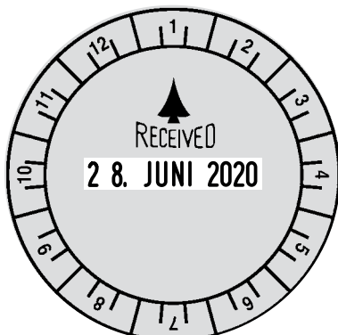
2910/U12 Ø 50mm | Max. text plate size 4mm | Date size
